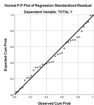
Gambar 1. Normal P-P Plot of Regression Standardized Residual
