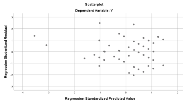
Gambar 1. Output Scatterplot
